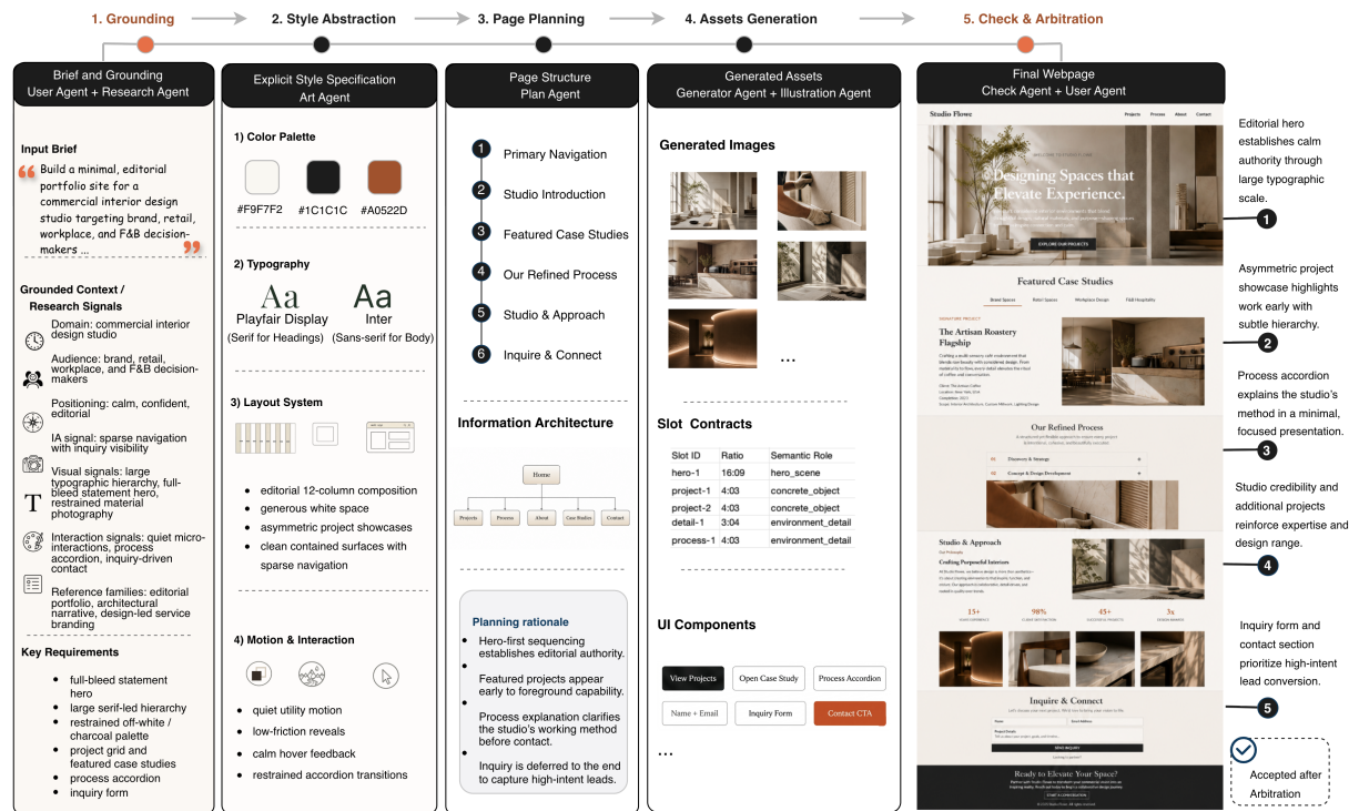
Figure 6: Appendix case study from Sample 000001. WebWeaver constructs an editorial architectural style contract and propagates it into a sparse portfolio webpage with controlled hierarchy, project browsing, and inquiry-oriented interaction.
