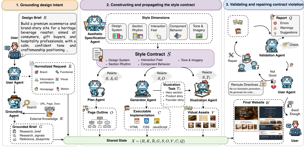
Figure 1: Overview of WebWeaver. The design-intent bottleneck is addressed by constructing a style contract from the grounded brief and propagating it through planning, asset generation, code synthesis, and validation.
