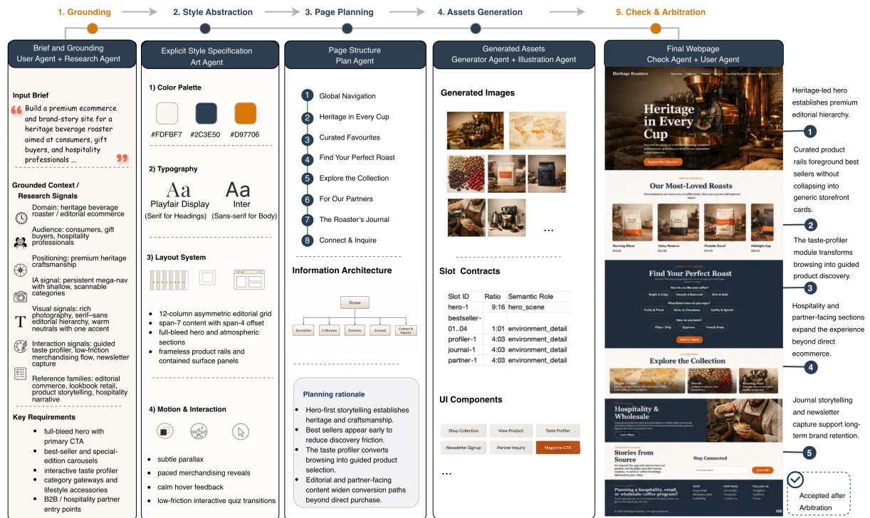
Figure 8: Appendix case study from Sample 000051. WebWeaver constructs an editorial heritage style contract and propagates it into coordinated merchandising, guided product discovery, brand storytelling, and front-end implementation.
