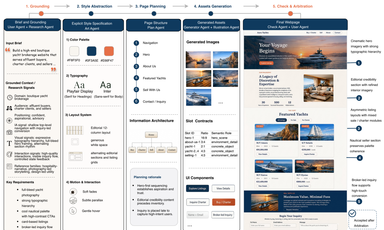
Figure 7: Appendix case study from Sample 000011. WebWeaver constructs a luxury yacht-brokerage style contract and propagates it into coordinated imagery, listing modules, and inquiry-oriented interaction.
