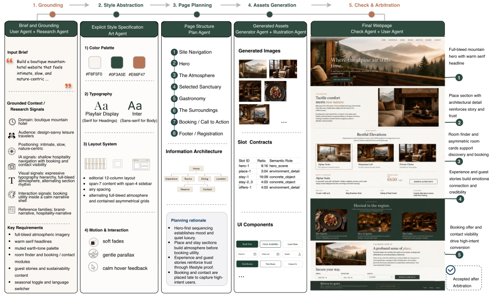
Figure 3: Case study from Web4Style sample 000061: WebWeaver propagates a boutique mountain-hotel style contract into page rhythm, visual assets, code, and booking interactions.
