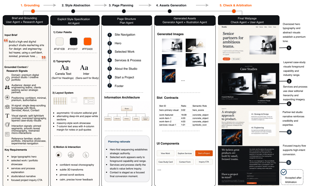
Figure 9: Appendix case study from Sample 000081. WebWeaver constructs a strategic-contrast style contract and propagates it into motion-aware pacing, portfolio storytelling, service explanation, and contact conversion.
