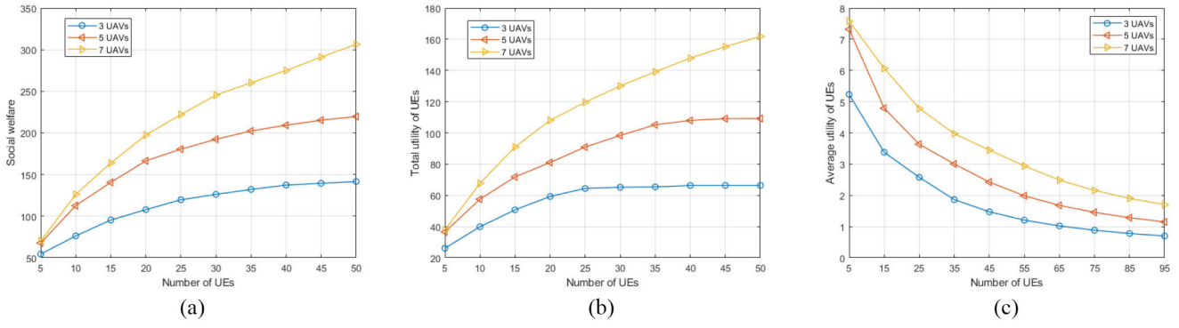
Fig. 7. Impact of the number of UAVs. (a) Impact of the number of UEs on social welfare for different numbers of UAVs. (b) Impact of the number of UEs on total utility of UEs for different numbers of UAVs. (c) Impact of the number of UEs on average utility of UEs for different numbers of UAVs.
