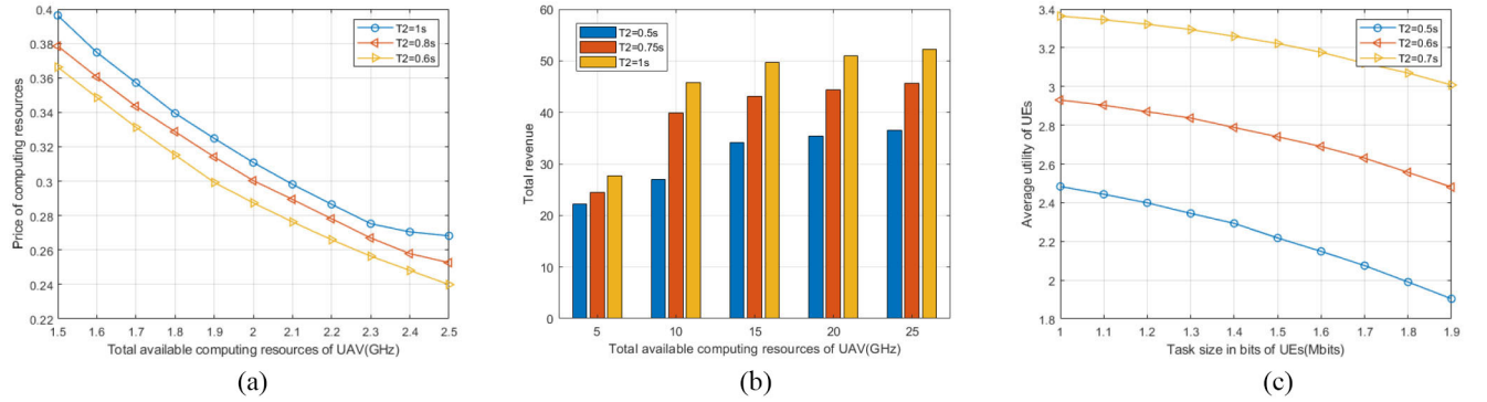
Fig. 6. Impact of maximum tolerated execution delay T_2 . (a) Impact of the total available computing resources on price of computing resources for different value of T_2 ( T_1 = 0.5 ). (b) Impact of the total available computing resources on total revenue for different value of T_2 ( T_1 = 0.5 ). (c) Impact of the task size in bits of UEs an average utility for different value of T_2 ( T_1 = 0.5 ).
