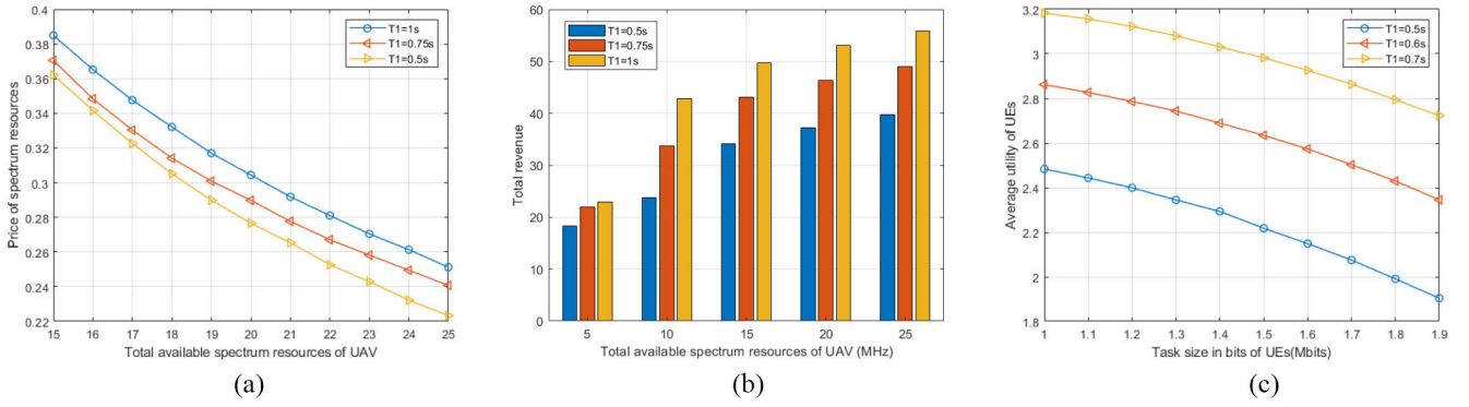
Fig. 5. Impact of maximum tolerated transmission delay T_1 . (a) Impact of the total available spectrum resources on price of spectrum resources for different value of T_1 ( T_2 = 0.6 ). (b) Impact of the total available spectrum resources on total revenue for different value of T_1 ( T_2 = 0.6 ). (c) Impact of the task size in bits of UEs an average utility for different value of T_1 ( T_2 = 0.6 ).
